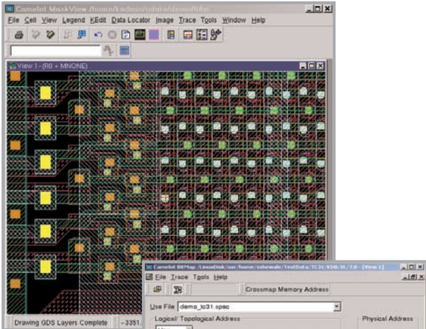
K-Bitmap identifies the physical location of bit addresses in memory devices
