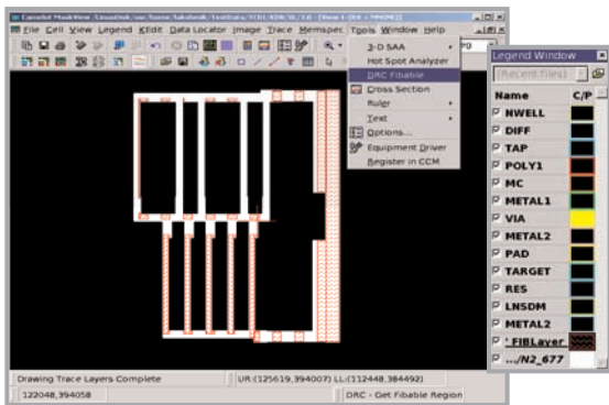
On-Line Search Analyzer finds easy-to-access traces
