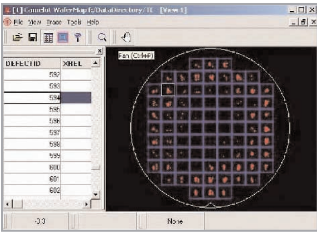
Defect Waver Map pinpoints defects for closer inspection and characterization
